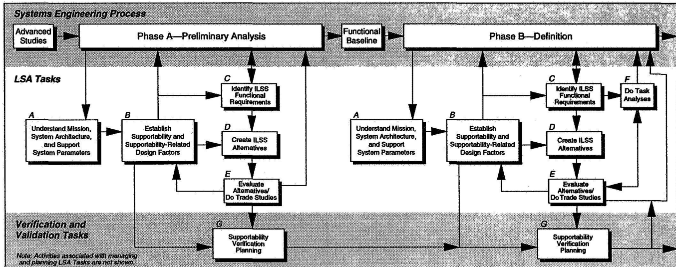
Figure 31a — Logistics Support Analysis Process Flow (Phases A and B).
