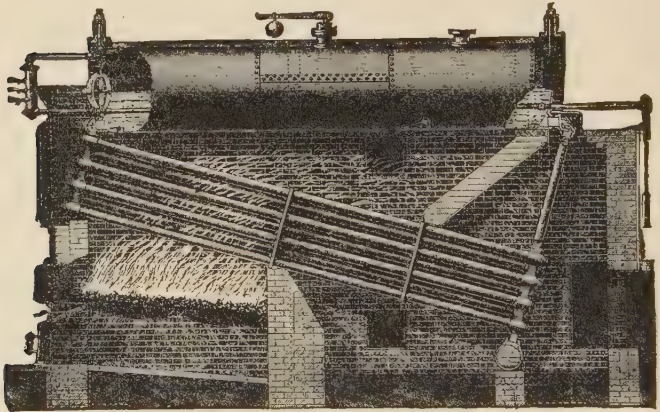
FIG. 112.—Babcock and Wilcox's Sectional Boiler.
