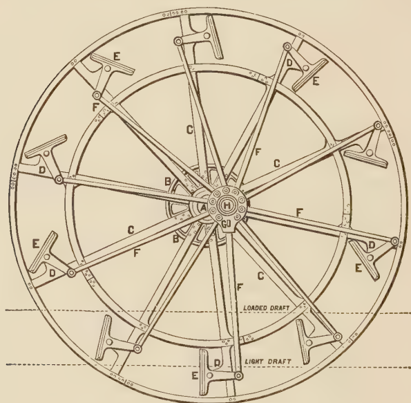
FIG. 87.—The Feathering Paddle-Wheel.
