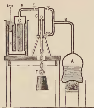
FIG. 25.—Watt's Experiment.
