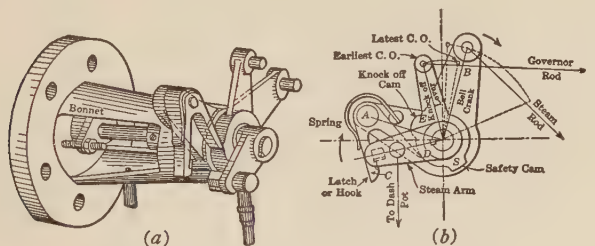
FIG. 158.—Reynolds Corliss Valve Gear.
