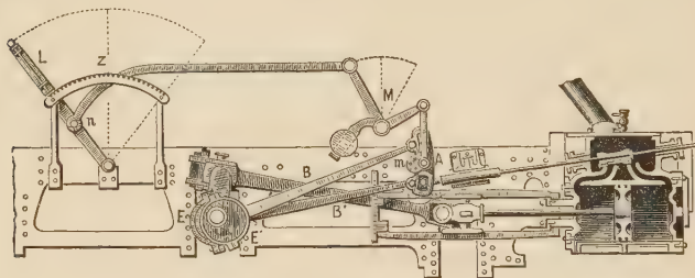
FIG. 53.—The Stephenson Valve-Gear, 1833.
