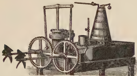
FIG. 84.—Engine, Boiler, and Screw-Propellers used by Stevens, 1804.
