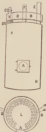
FIG. 74.—Read's Multi-Tubular Boiler, 1788.
