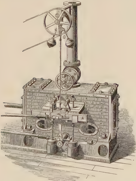
FIG. 99.—Greene Engine.
