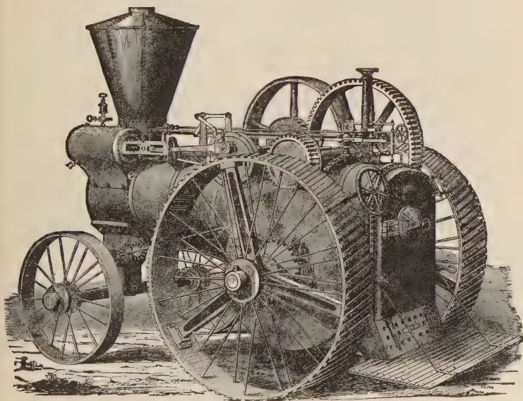
FIG. 117.—The Thrashers' Road-Engine, 1879.
