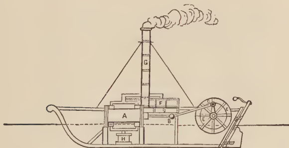
FIG. 75.—The "Charlotte Dundas," 1801.
