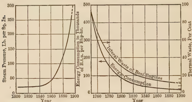
FIG. 172.—Rise in Steam Pressures, 1800–1897.
