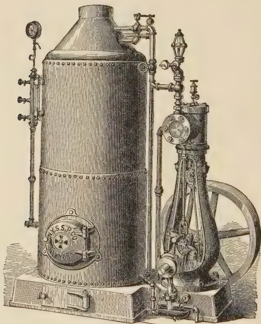
FIG. 114.—Semi-Portable Engine, 1878.
