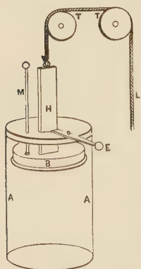
FIG. 17.—Papin's Engine.
