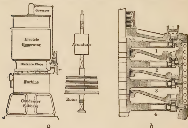
FIG. 180.—Arrangement of Curtis Vertical Turbine.
