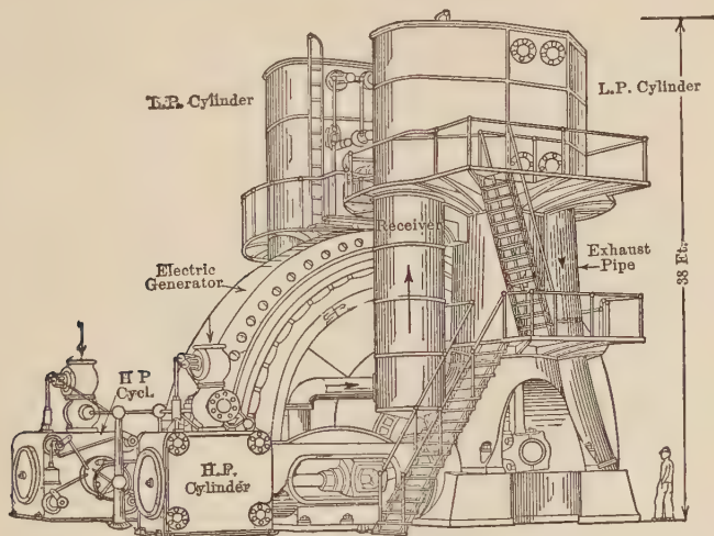
FIG. 160.—"Manhattan Engine."
