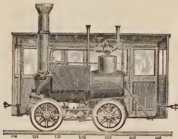
FIG. 125.—Tank-Engine, New York Elevated Railroad.
