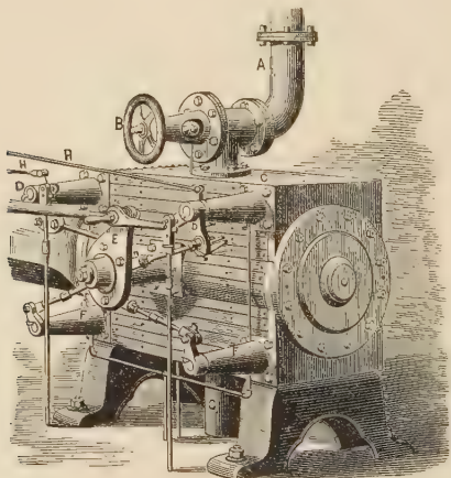
FIG. 98.—Corliss Engine Valve-Motion.
