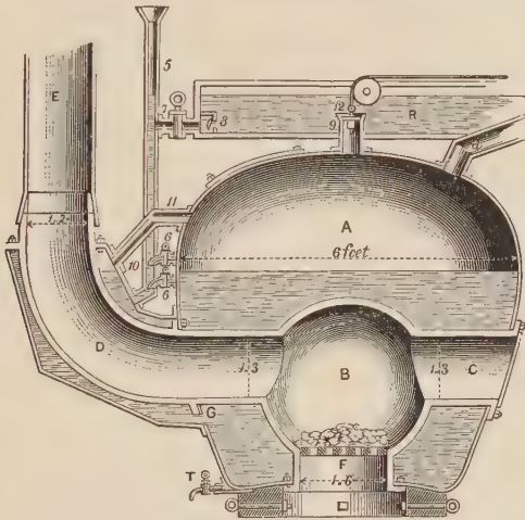
FIG. 23.—Smeaton's Portable-Engine Boiler, 1765.
