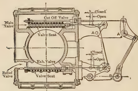
FIG. 165.—Valves of the McIntosh-Seymour Engine.
