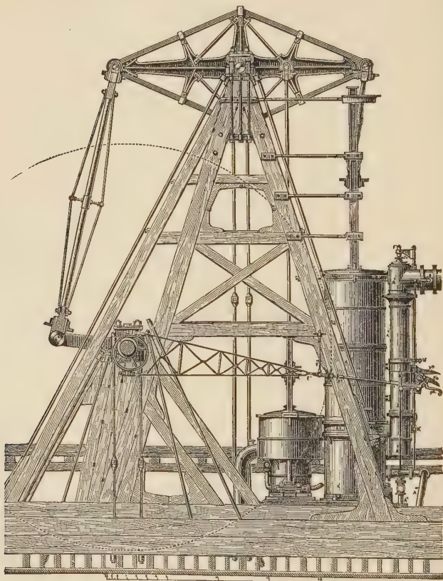
FIG. 130.—Beam-Engine.
