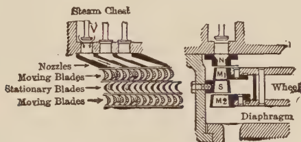
FIG. 179.—Velocity Compounding—Curtis Type.
