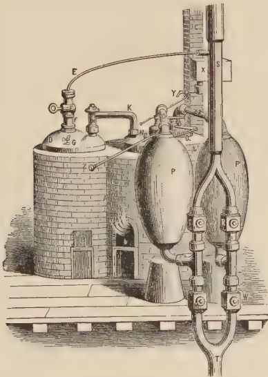
FIG. 18.—Savery's Engine, A. D. 1702.
