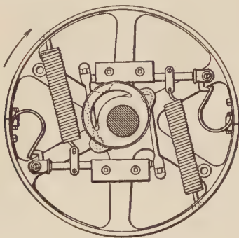
FIG. 164.—Thompson (Buckeye) Governor.
