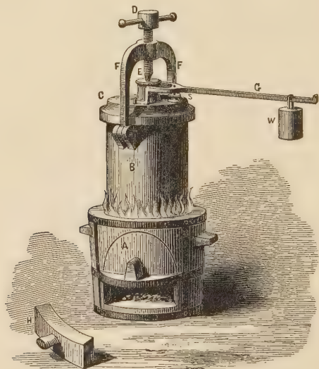
FIG. 16.—Papin's Digester, 1680.
