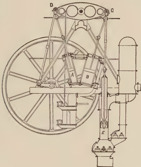
FIG. 107.—The Leavitt Pumping-Engine.
