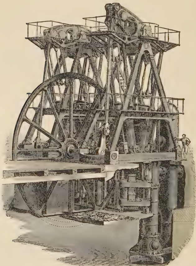
FIG. 106.—The Lawrence Water-Works Engine.
