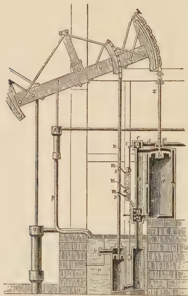
FIG. 26.—Watt's Engine, 1774.
