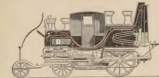
FIG. 48.—Gurney's Steam-Carriage.
