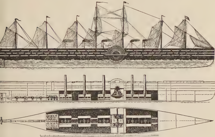
FIG. 146.—The Great Eastern.
