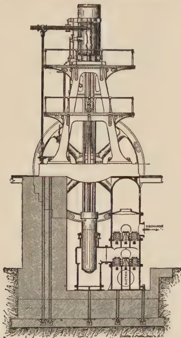
FIG. 170.—Typical Arrangement of Multiple-Expansion Pumping Engine.
