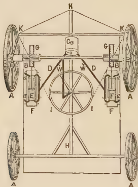
FIG. 43.—Read's Steam-Carriage, 1790.
