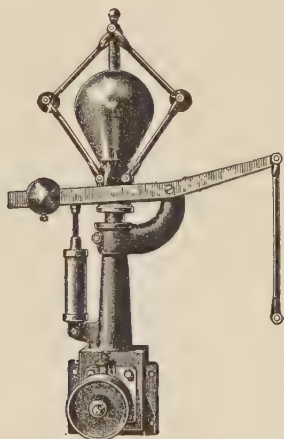
FIG. 161.—Porter Loaded Governor.
