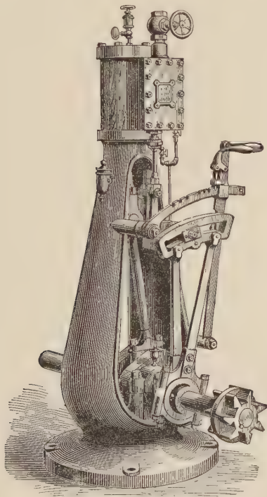
FIG. 135.—Launch-Engine.
