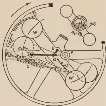
FIG. 168.—Inertia Type of Shaft Governor (Rites).
