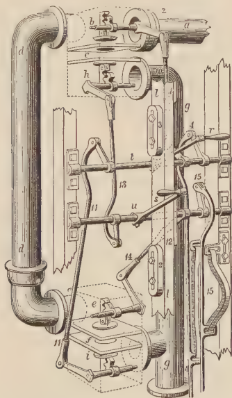
FIG. 82.—Valve-Gear of the Albion Mills Engine.
