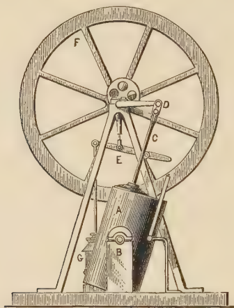
FIG. 36.—Murdoch's Oscillating Engine, 1785.
