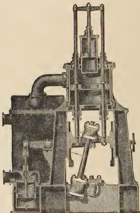
FIG. 155.—Tandem Compound Engine. (Scale \frac{1}{8} .)
