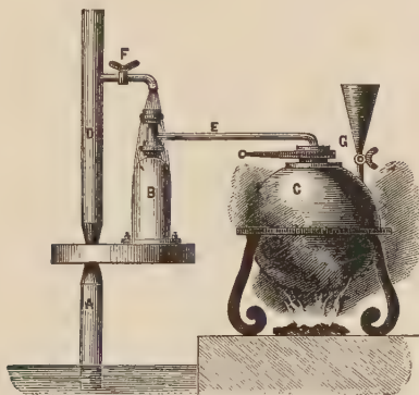
FIG. 12.—Savery's Engine, 1698.
