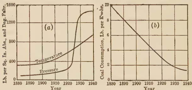
FIG. 182.—Progress in Pressures, Temperatures and Coal Consumption, 1880-1939.
