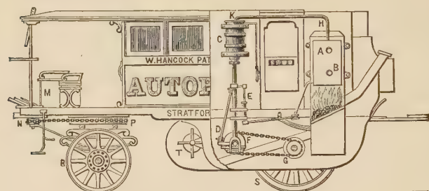
FIG. 49.—Hancock's "Autopsy," 1833.
