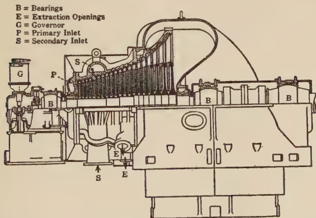
FIG. 181.—Typical Arrangement of Large General Electric Turbine.
