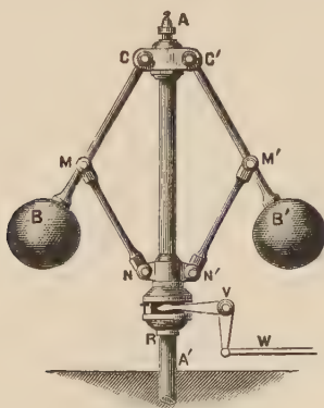
FIG. 29.—The Governor.
