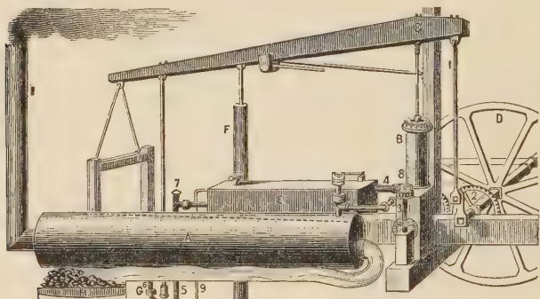
FIG. 46.—Evans's Non-condensing Engine, 1800.
