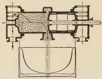
FIG. 171.—Cylinder of the Stumpf Uniflow Engine.
