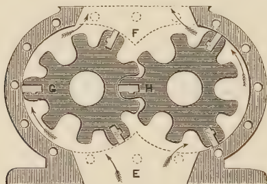
FIG. 124.—Rotary Pump.
