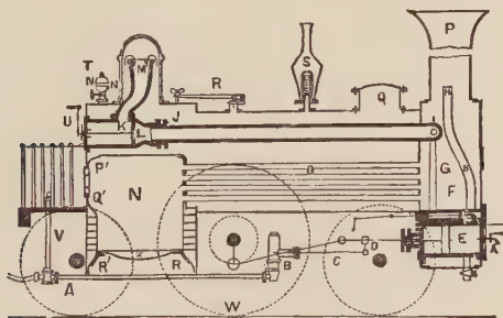
FIG. 127.—British Express Engine.
