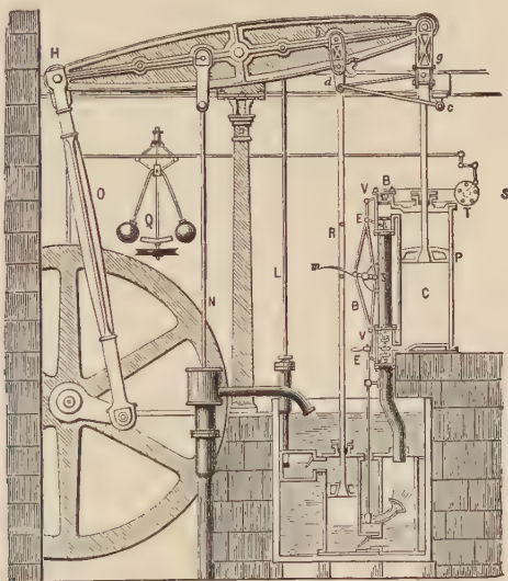
FIG. 31.—Boulton & Watt's Double-Acting Engine, 1784.
