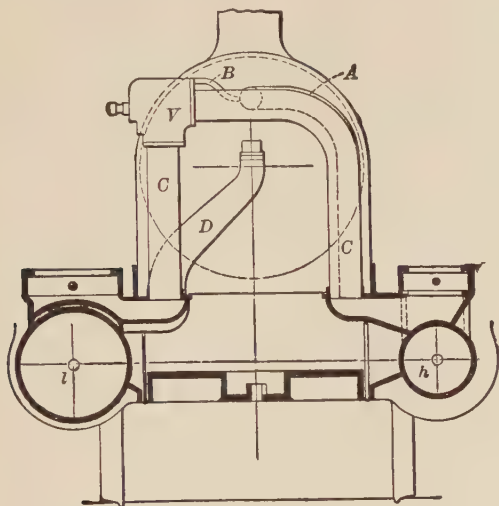
FIG. 149.—Compound Engine.
