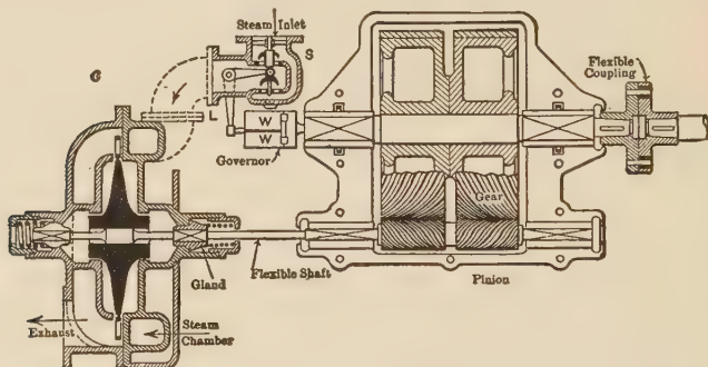
FIG. 178.—Elements of a Small de Laval Turbine.
