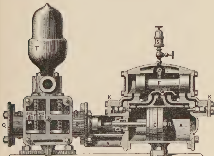
FIG. 102.—Steam-Pump.
