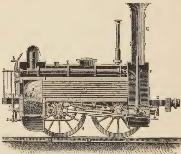
FIG. 57.—Stephenson's Locomotive, 1833.
