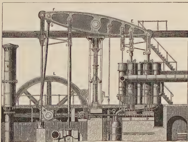
FIG. 105.—Double-Cylinder Pumping-Engine, 1873.
