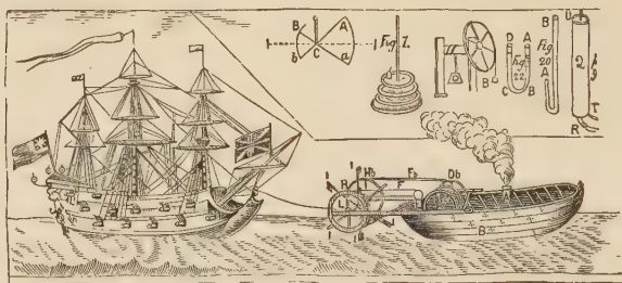
FIG. 66.—Hulls's Steamboat, 1736.
