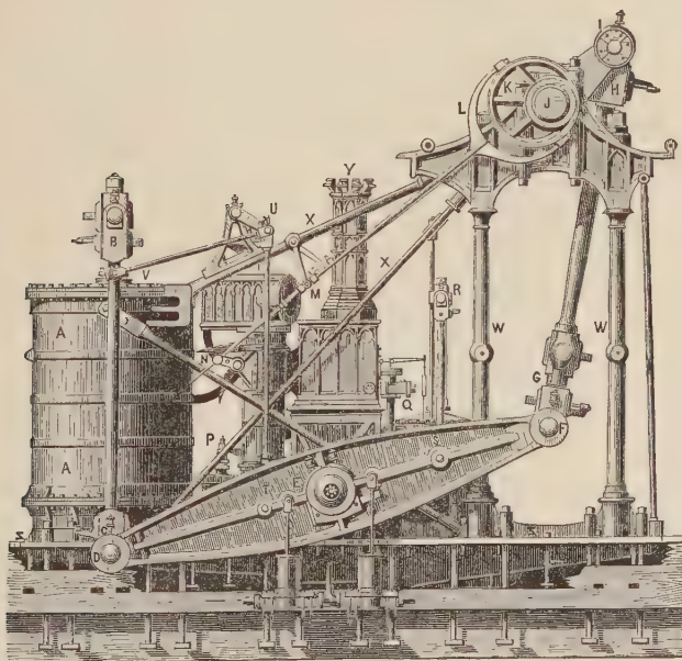
FIG. 92.—The Side-Lever Engine, 1849.
