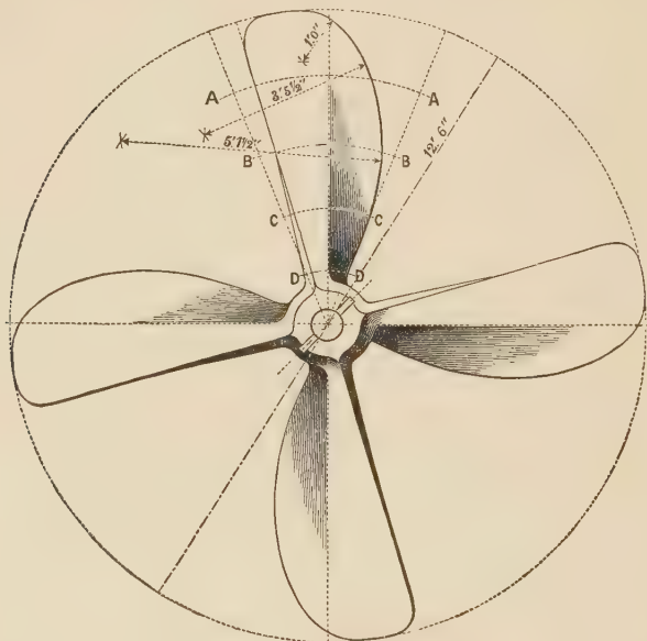
FIG. 139.—Screw-Propeller.
