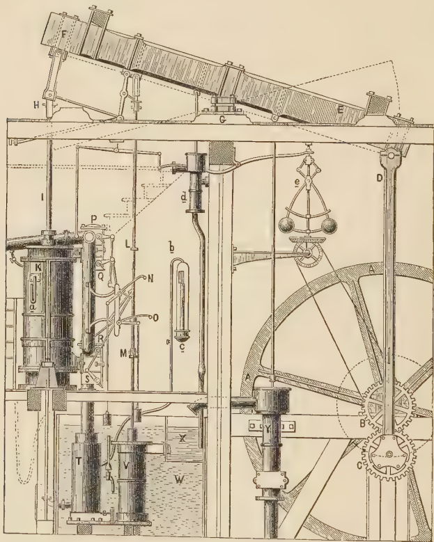
FIG. 27.—Watt's Engine, 1781.
