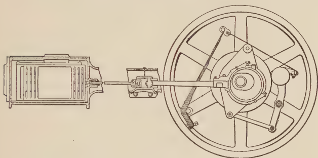
FIG. 167.—Sweet Governor, Swinging Eccentric and Valve Gear.
