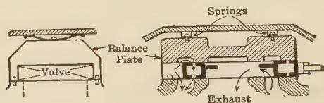
FIG. 166.—Sweet Valve and Balance Plate.
