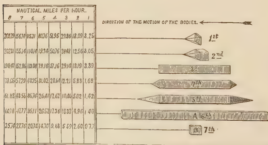
FIG. 78.—Fulton's Table of Resistances.
