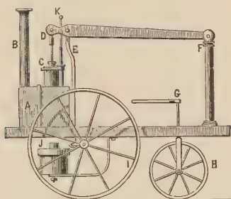
FIG. 45.—Murdoch's Model, 1784.
