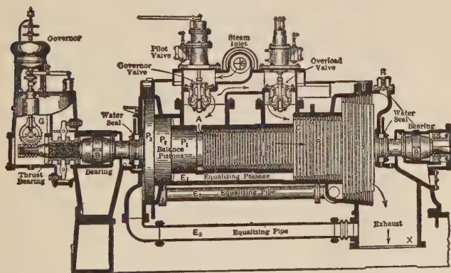
FIG. 175.—Elements of an Early Westinghouse-Parsons Turbine.
