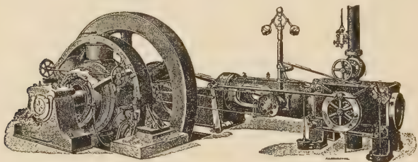
FIG. 159.—Reynolds Heavy Duty Corliss Engine, with Direct Connected Electric Generator (1890).
