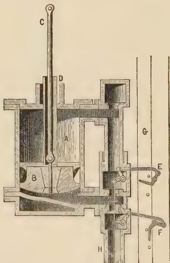
FIG. 33.—Watt's Half-Trunk Engine, 1784.
