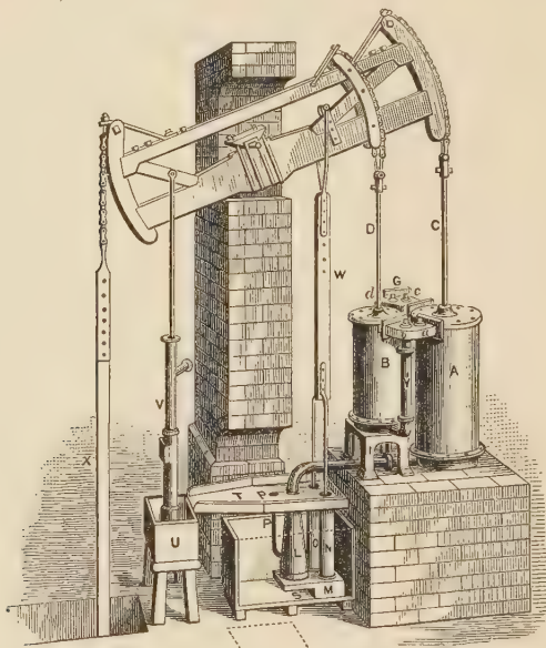
FIG. 37.—Hornblower's Compound Engine, 1781.
