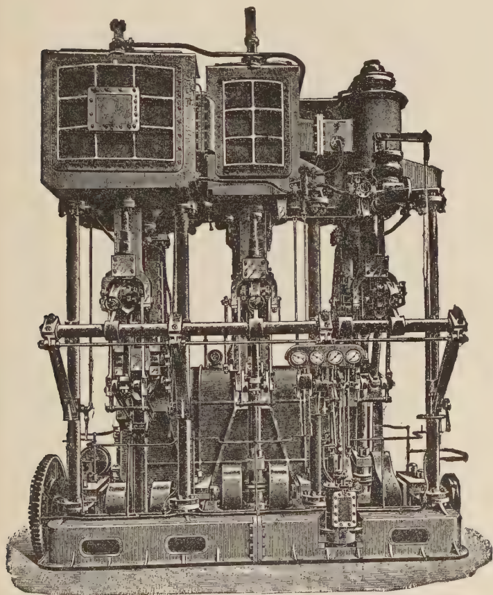
FIG. 156.—Triple-expansion Engine.
