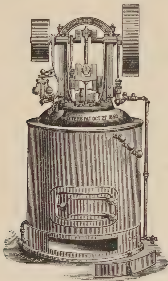
FIG. 115.—Semi-Portable Engine, 1878.
