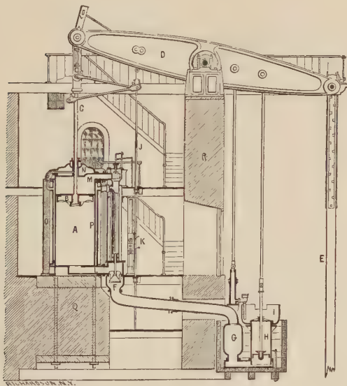
FIG. 101.—Cornish Pumping-Engine, 1880.
