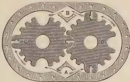
FIG. 123.—Rotary Steam-Engine.
