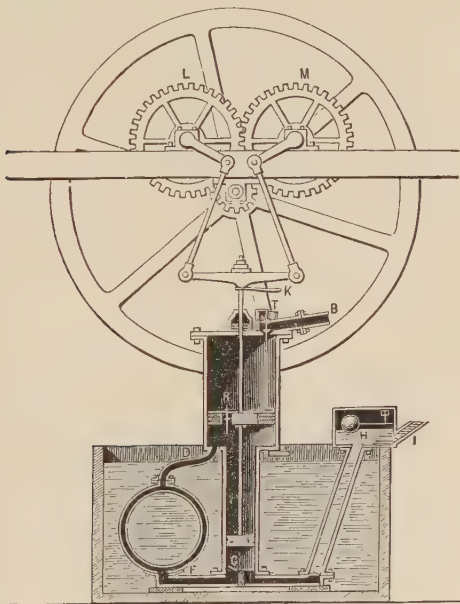
FIG. 89.—Cartwright's Engine, 1798.
