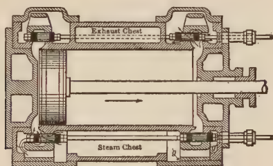
FIG. 163.—Porter-Allen Steam Cylinder.
