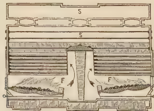
FIG. 143.—Marine High-Pressure Boiler. Section.
