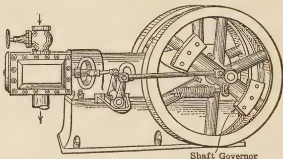
FIG. 169.—High-Speed, Single-Valve, Center-Crank Engine with Inertia Governor.
