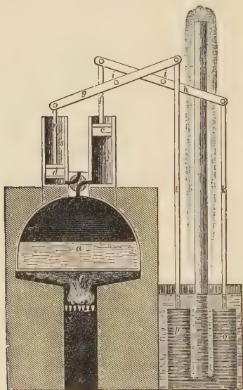
FIG. 41.—Leupold's Engine, 1720.
