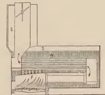
FIG. 89.—Stevens's Return Tubular Boiler, 1832.
