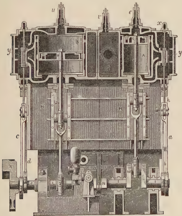
FIG. 138.—Compound Marine Engine. Front Elevation and Section.
