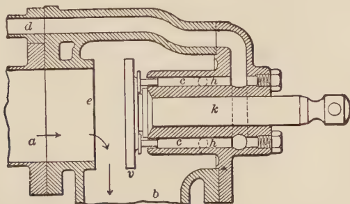
FIG. 150.—"Intercepting Valve."
