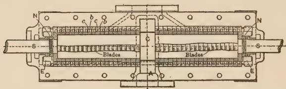
FIG. 174.—Parsons' First Turbine.
